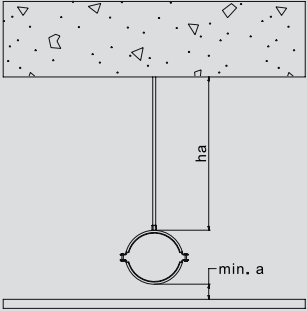
FRS-F pipe clamps – load table based on the advisory opinion no. GS 3.2/14-175-2
