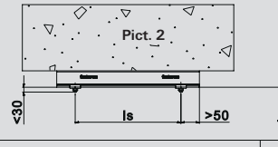
FLS-Channel / ALK-Cantilever arm - load table based on the advisory opinion no. GS 3.2/15-141-4
