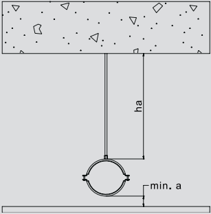
Pipe clamp FRS-L Universal - load table based on the advisory opinion no. GS 3.2/15-141-3
